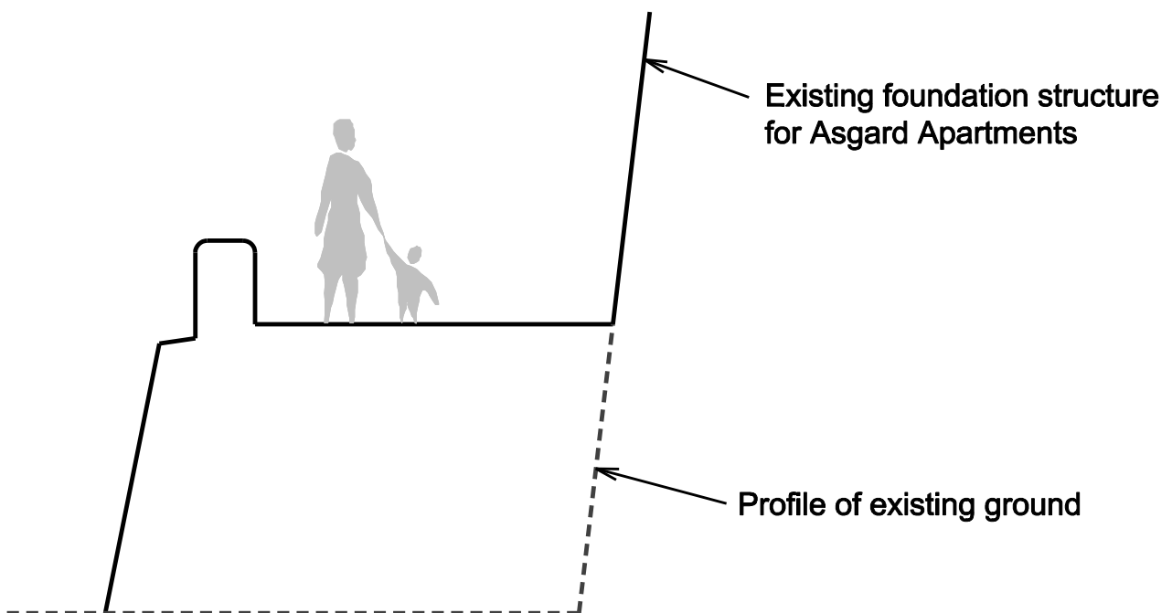
Typical Section: Proposed boardwalk 3m width
