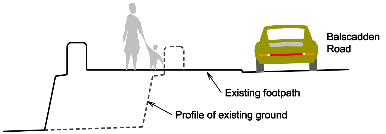
Typical Section: Proposed combined boardwalk/footpath 4m width
